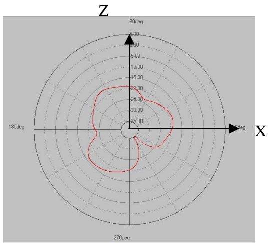
Peak Gain -16.17dBi
